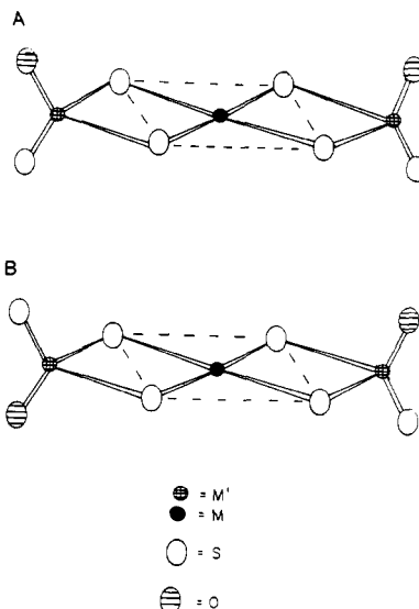
Figure 1. Possible structures of \text{M}(\text{M}'\text{OS}_3)_2^{2-} complexes: A, cis isomer; B, trans isomer.
