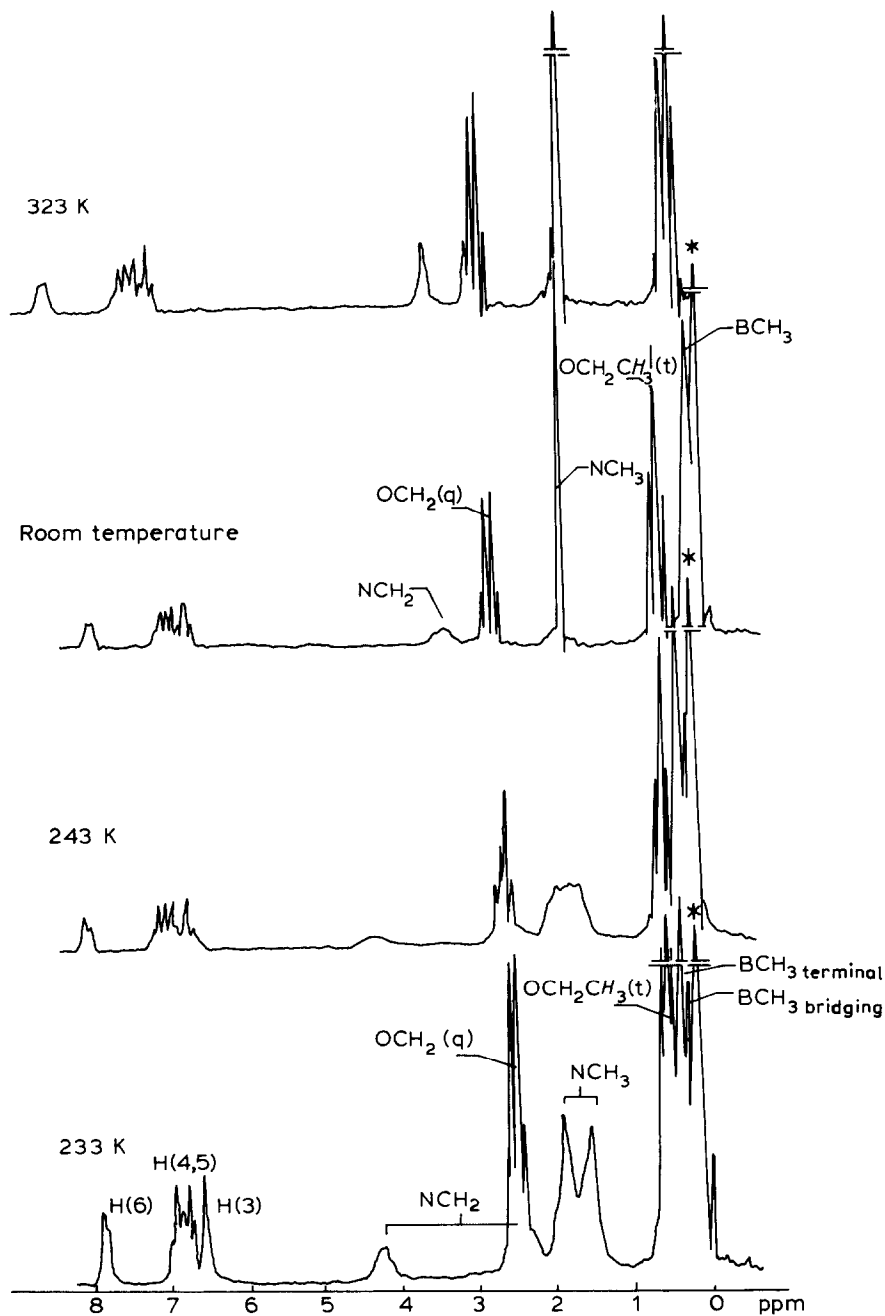
Fig. 1. ^1\text{H} NMR spectra ( \delta , ppm) of (\text{ArBMe}_3)\text{Li}\cdot\text{OEt}_2 in \text{toluene-}d_8 , at various temperatures, \star internal TMS signal.
