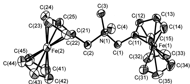
Fig. 2. ORTEP drawing of the cation (\text{FcCH}_2)_2\text{NMe}_2^+ in the \text{SbF}_6^- salt 1b with 30% thermal ellipsoids. Hydrogen atoms are omitted.
