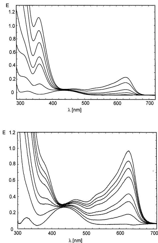
Fig. 7. UV-vis traces during the oxidation of the \text{FcCH}_2\text{NMe}_2\text{H}^+ ion (top) and the (\text{FcCH}_2)_2\text{NMe}_2^+ ion (bottom) in an OTTLE cell. In both cases the lowest curve represents the spectra before oxidation and the uppermost trace the spectra after complete oxidation to the ferrocenium ions.
