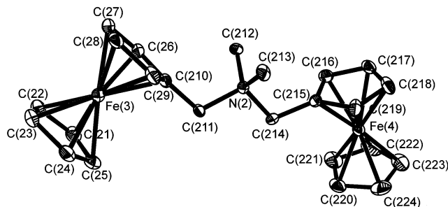
Fig. 3. ORTEP drawing of one of the three independent cations of (\text{FcCH}_2)_2\text{NMe}_2^+ in the \text{Cl}^- salt 1d ·4/3 \text{H}_2\text{O} (cation 2) with 30% thermal ellipsoids. Hydrogen atoms are omitted.
