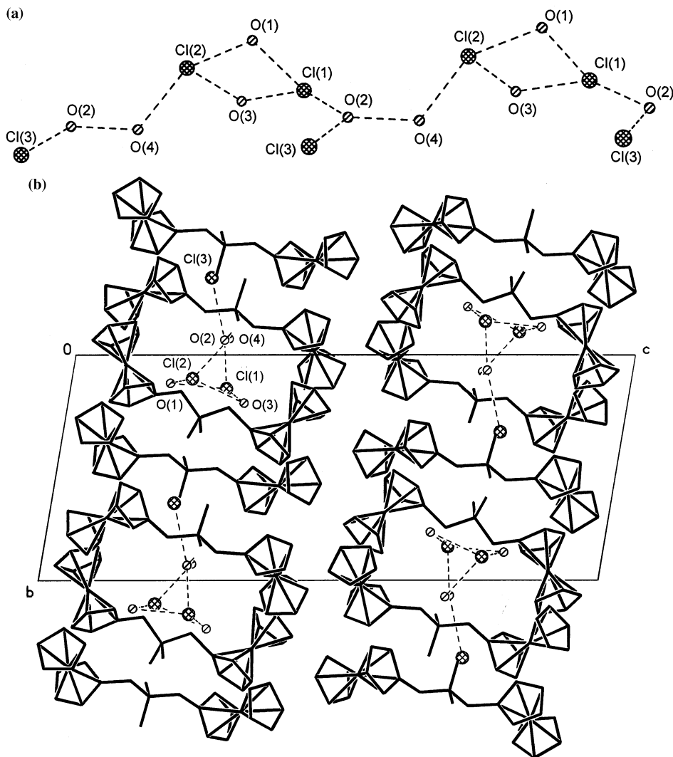
Fig. 4. (a) View of a one dimensional chain comprised of hydrogen bonded \text{Cl}^- and \text{H}_2\text{O} in the structure of 1\mathbf{d} \cdot 4/3\text{H}_2\text{O} . (b) Packing diagram of (1\mathbf{d} \cdot 4/3\text{H}_2\text{O}) . One of the \text{Cl}^- ions is statistically replaced by \text{CN}^- (not shown).
