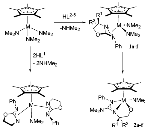
Scheme 1. Synthesis of Half-Sandwich Aminooxazolate Complexes
