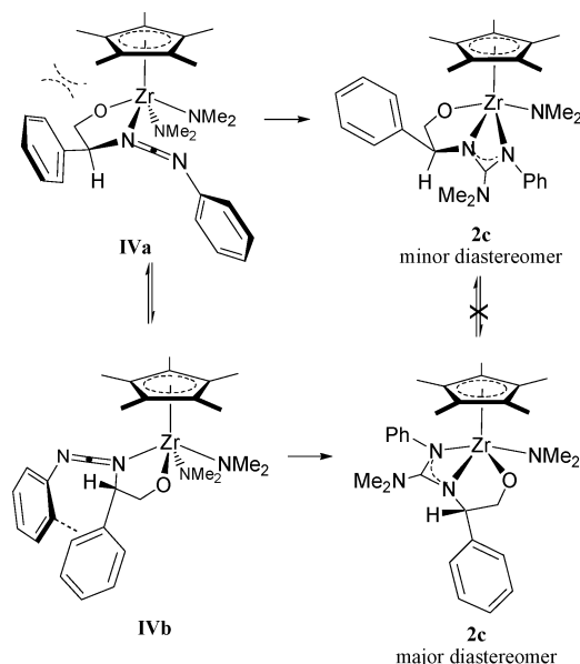
Scheme 3. Origin of Diastereoselection in the Formation of 2c
