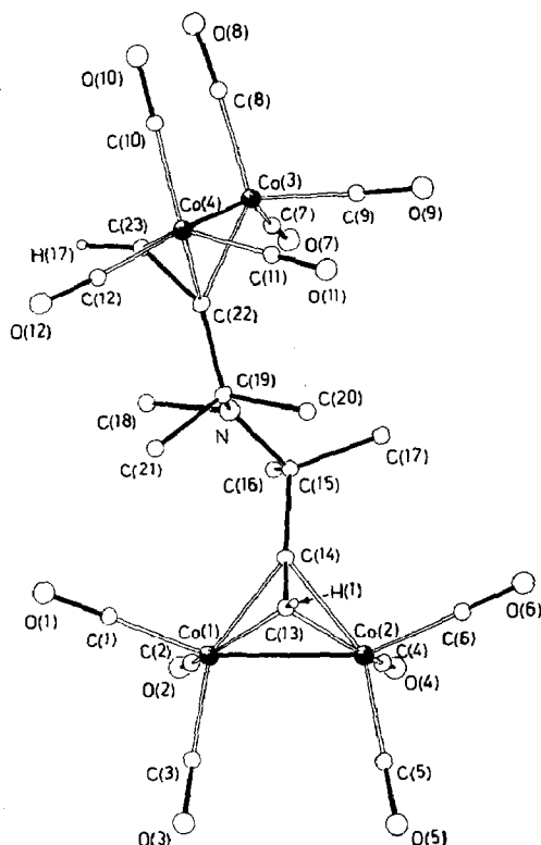
Fig. 1. Perspective view of the [\text{Co}_2(\text{CO})_6]_2\text{N-McTMDPA} molecule.
