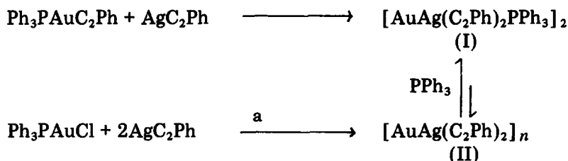
SCHEME 1. A reaction product of route a is [\text{Ph}_3\text{PAgCl}]_4 .
