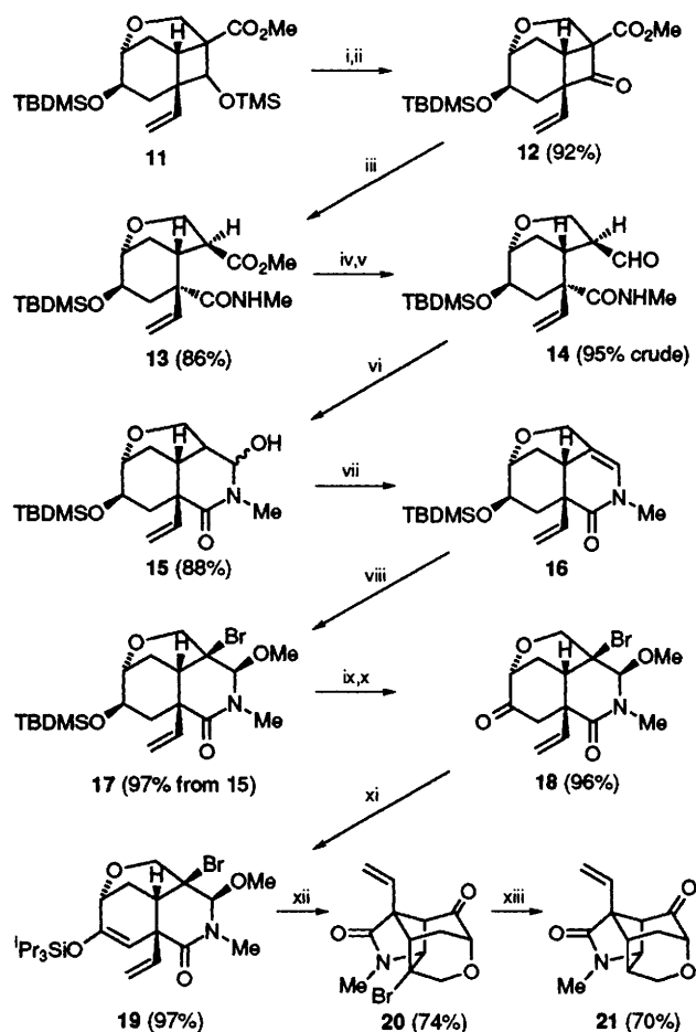
Scheme 4 Reagents and conditions: i, K_2CO_3 , MeOH, THF; ii, (a) Me_2SO , TFAA, -70^\circ C , (b) Et_3N ; iii, MeNH_2 , MeOH, THF; iv, LiBH_4 , MeOH, Et_2O ; v, CrO_3 , pyridine, DCM; vi, K_2CO_3 , MeOH; vii, TsOH , DCM; viii, Br_2 , MeOH; ix, Bu_4NF , THF; x, (a) Me_2SO , (COCl)_2 , (b) Et_3N ; xi, Pr_3SiOTf , Et_3N ; xii, TFA, reflux, 15 min; xiii, Bu_3SnH , benzene, reflux
