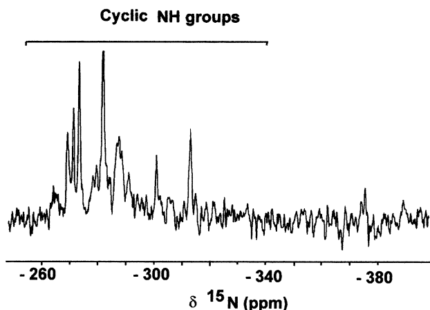
Fig. 2. ^{15}\text{N} -NMR spectrum at the end of the co-polymerisation reaction.
