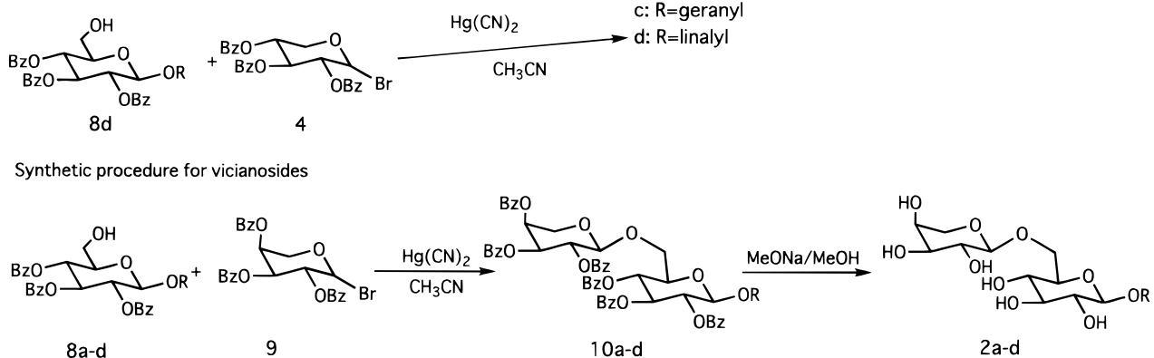
Figure 1. General synthetic procedures for primeverosides and vicianosides.
