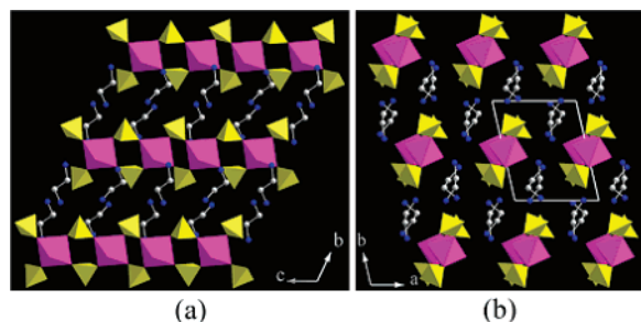
Figure 3. Views of the structure of 1 (a) along the [1\ 0\ 0] direction and (b) along the [0\ 0\ 1] direction: \text{PO}_4 , yellow tetrahedra; \text{NbO}_5\text{F} , purple octahedra.
