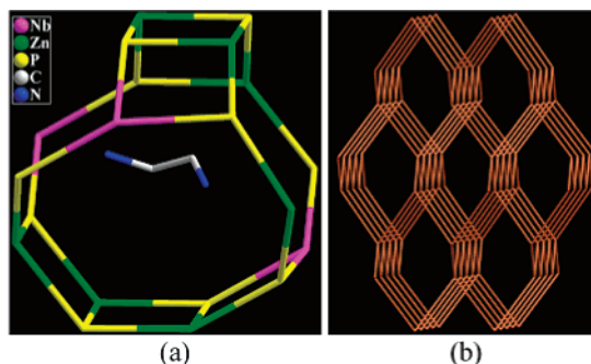
Figure 6. (a) [4 6 8 4 ] cage encapsulating an ethylenediamine in 2 . Oxygen atoms and the disordered parts of ethylenediamine are omitted for clarity. (b) Net (6·6·6·6 2 ·6 2 ·6 2 ) of [4 6 8 4 ] cage centers in 2 related to diamond net (6 2 ·6 2 ·6 2 ·6 2 ·6 2 ).
