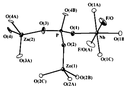
Figure 4. ORTEP plot of the asymmetric unit showing the local coordination environments of cations in compound 2 , with the symmetry-related part drawn as open circles. Thermal ellipsoids are given at 30% probability.
