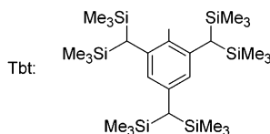
Scheme 1. Synthesis of 1 a
