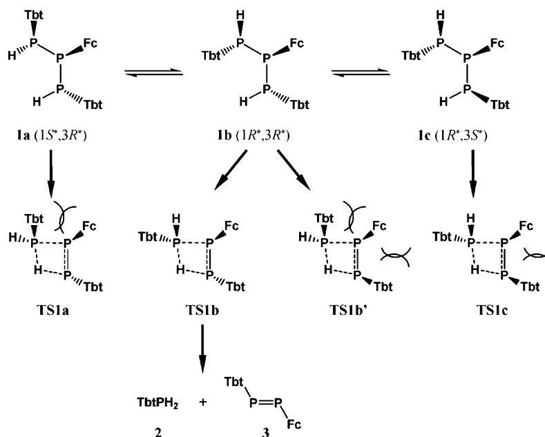
Scheme 4. Possible Mechanism for the Thermolysis of 1
