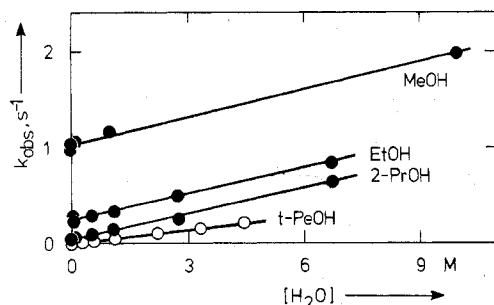
Figure 1. Effect of water on k_{obsd} at constant ligand concentration ( [Cu(SA=N-t-Bu)_2] = 5 \times 10^{-4} M ; [HSA=N-Et] = 0.02 M (MeOH), 0.01 M (EtOH, 2-PrOH), 0.005 M ( t -PeOH = tert-pentyl alcohol = 2-methyl-2-butanol); T = 298 K ).
