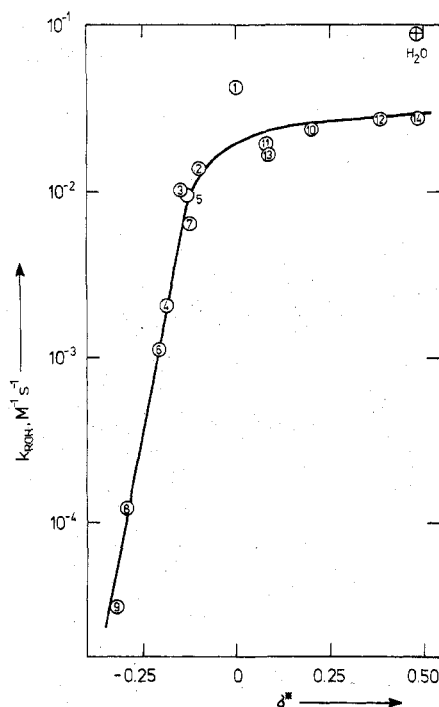
Figure 2. Plot of k_{\text{ROH}} vs. \sigma^* (Taft) (the numbers refer to the solvents listed in Tables II and III).
