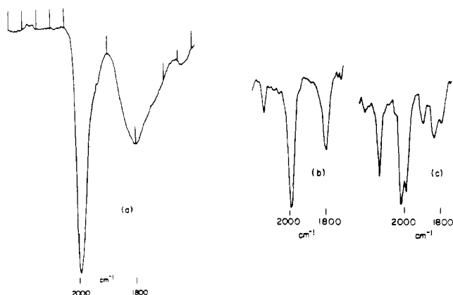
Figure 7. Infrared spectra of [\text{Rh}_{10}\text{As}(\text{CO})_{22}]^{3-} in solutions of sulfolane (tetrahydrothiophene 1,1-dioxide): (a) at ambient conditions; (b) under 537 atm of \text{CO-H}_2 at 150 °C; (c) under 862 atm of \text{CO-H}_2 at 150 °C.
