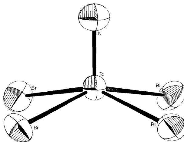
Fig. 5. ORTEP plot of the complex anion in (\text{Ph}_4\text{As})\text{TcNBr}_4 .
