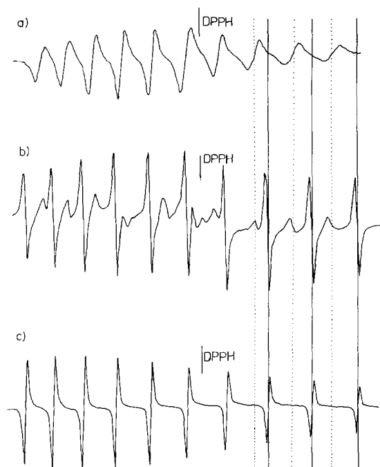
Fig. 4. Room temperature EPR spectra of a reaction mixture during the thermal decomposition of [\text{Tc}(\text{NS})\text{Cl}_4]^- : (a) immediately after dissolving the starting compound (only the signals of [\text{Tc}(\text{NS})\text{Cl}_4]^- can be observed), (b) after standing for 24 h at room temperature (the signals of [\text{Tc}(\text{NS})\text{Cl}_4]^- and [\text{TcNCl}_4]^- can be observed), (c) after additional refluxing for 10 min (only the signals of [\text{TcNCl}_4]^- can be observed).
