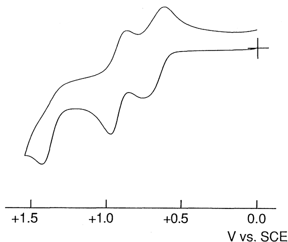
Figure 1. Cyclic voltammogram of 1c in benzonitrile-carbon disulfide (1:1, v/v).
