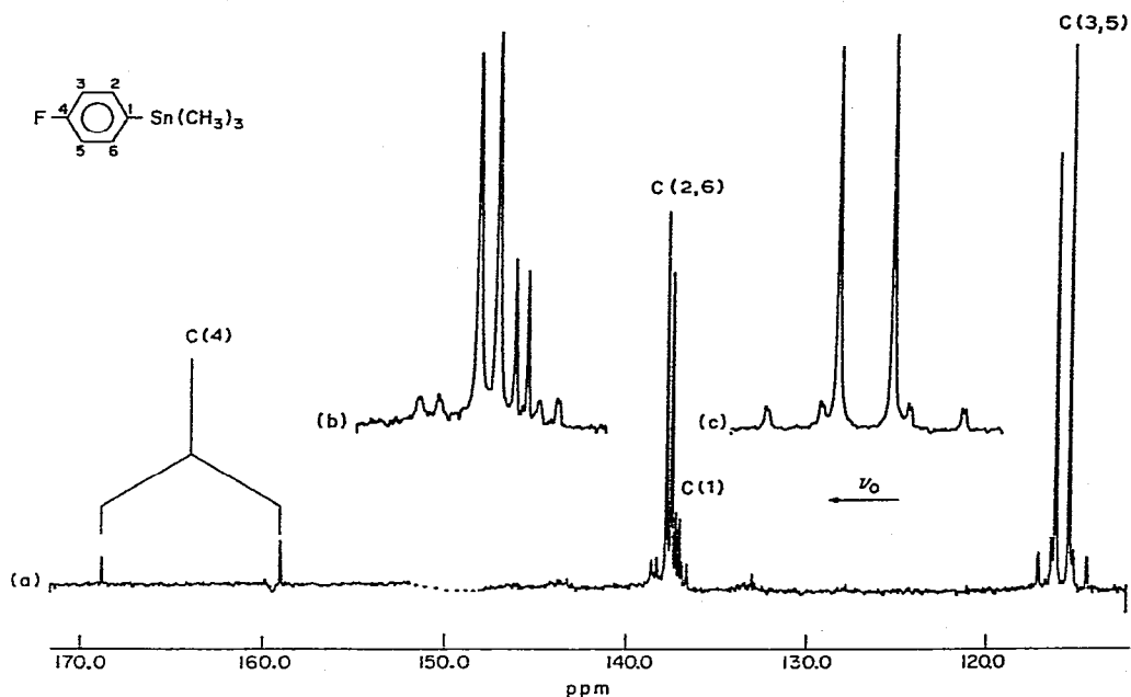
Fig. 1. (a) Aromatic carbons of para -fluorophenyltrimethyltin showing ^{13}\text{C} - ^{19}\text{F} couplings (see Table 7). Scale is in ppm downfield from internal TMS. This proton noise-decoupled spectrum required 6000 pulses, using 16384 data points with a collection time of 4.1 s per pulse. The pulse width was 20 \mu\text{s} . Phase of sample: neat liquid. Dotted line at ca. 150 ppm indicates region of folded peak. (b) Region of C(2, 6) (left) and lower intensity C(1) carbon resonances. Conditions same as for (a), but region is four-fold expanded. (c) Region of C(3, 5) carbon resonance. Fluorine-split \text{Sn} - ^{13}\text{C} satellites are clearly resolved into 117, 119 components, as in (b). Conditions same as for (b).
