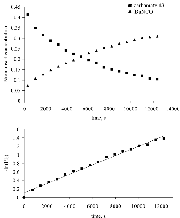
Figure 5. (a, top) Plot of normalized concentrations vs time for the 'BuNCO extrusion reaction of [\text{Ti}(\eta\text{-C}_5\text{H}_4\text{Me})\{\text{N}^+\text{BuC}(\text{O})\text{O}\}\{\text{Me}_3\text{SiNC}(\text{Ph})\text{NCH}_2\text{CH}_2\text{CH}_2\text{NMe}_2\}] ( 13 ). Values given are for the carbamate 13 and 'BuNCO. (b, bottom) Plot of \ln(I/I_0) vs time for the 'BuNCO extrusion reaction of [\text{Ti}(\eta\text{-C}_5\text{H}_4\text{Me})\{\text{N}^+\text{BuC}(\text{O})\text{O}\}\{\text{Me}_3\text{SiNC}(\text{Ph})\text{NCH}_2\text{CH}_2\text{CH}_2\text{NMe}_2\}] ( 13 ).
