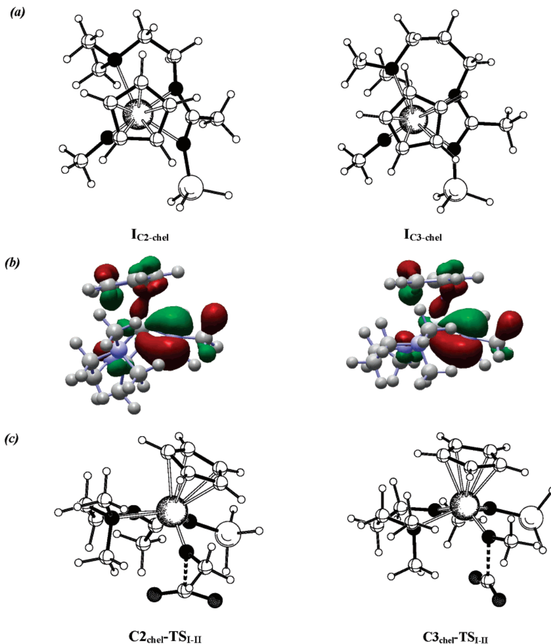
Figure 9. (a) DFT minimized geometries of the chelated imido amidinate complexes \text{IC}_{2\text{-chel}} (left) and \text{IC}_{3\text{-chel}} viewed along the \text{Cp}_{\text{cent}} \cdots \text{Ti} vectors. (b) Representations of the HOMO of each compound viewed approximately perpendicular to these vectors. (c) Geometries of the transition states for \text{CO}_2 cycloaddition to \text{Ti}=\text{NMe} ( \text{C}_{2\text{chel}}\text{-TS}_{\text{I-II}} for addition to \text{IC}_{2\text{-chel}} and \text{C}_{3\text{chel}}\text{-TS}_{\text{I-II}} for addition to \text{IC}_{3\text{-chel}} ).
