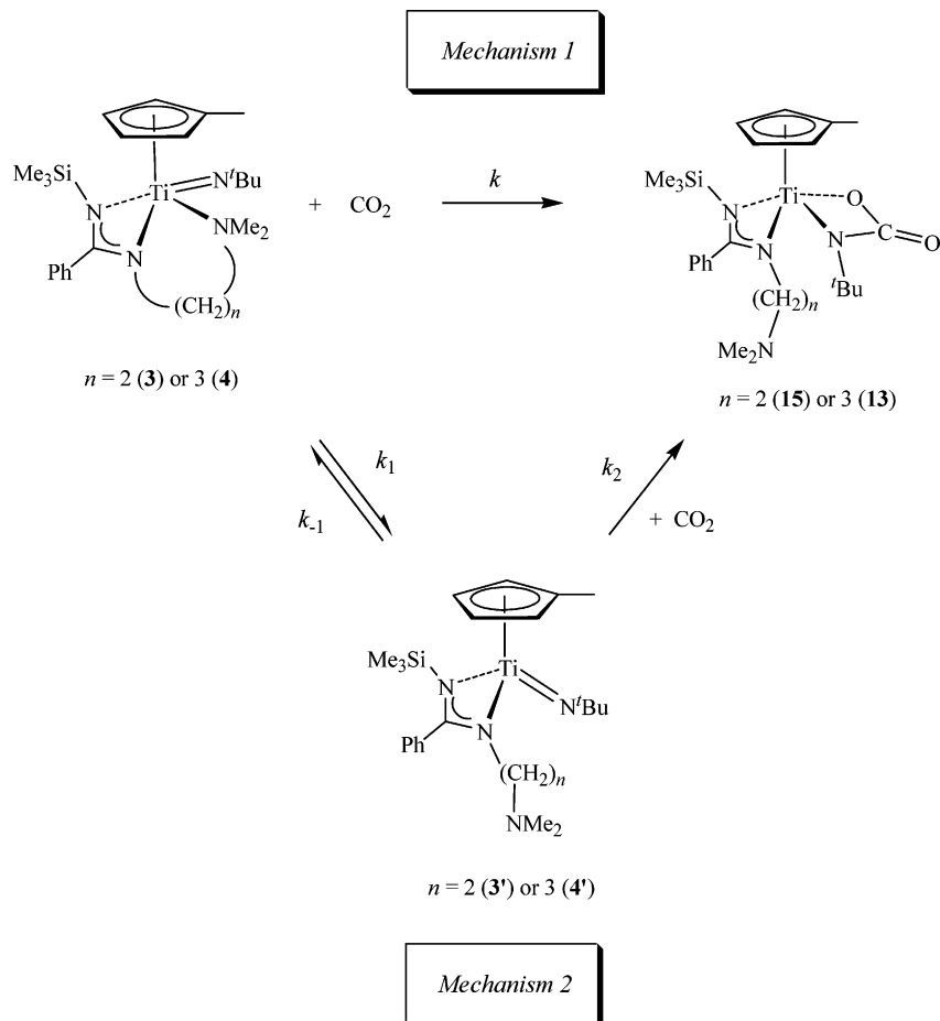
Scheme 4. Two Alternative Mechanisms for the Formation of Carbamates 15 and 13 from the Starting Imido Complexes 3 or 4 on Reaction with CO 2 : (Mechanism 1) Cycloaddition at the Complex with the NMe 2 Group Coordinated; (Mechanism 2): Dissociation of NMe 2 Precedes Cycloaddition
