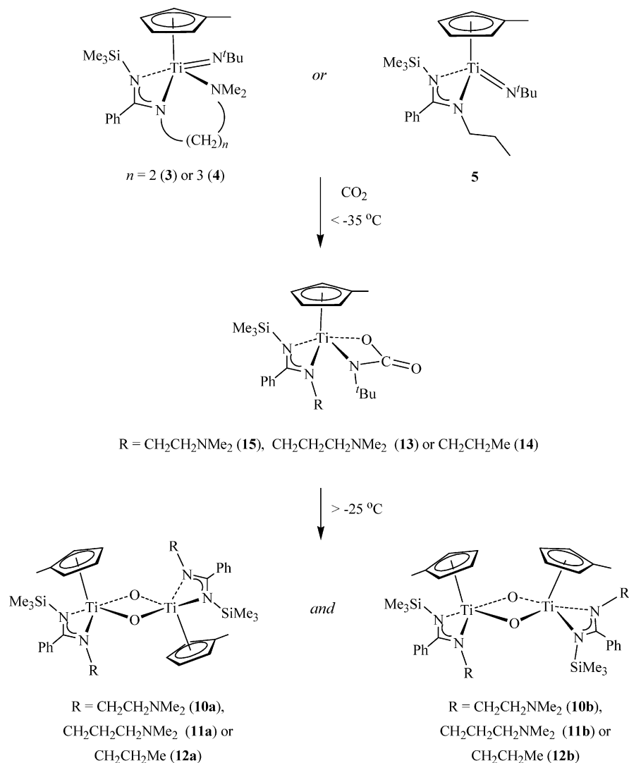
Scheme 3. Reactions of [\text{Ti}(\eta\text{-C}_5\text{H}_4\text{Me})(\text{N}^t\text{Bu})\{\text{Me}_3\text{SiNC(Ph)N(CH}_2)_n\text{NMe}_2\}] ( n = 2 ( 3 ), 3 ( 4 )) and [\text{Ti}(\eta\text{-C}_5\text{H}_4\text{Me})(\text{N}^t\text{Bu})\{\text{Me}_3\text{SiNC(Ph)NCH}_2\text{CH}_2\text{Me}\}] ( 5 ) with \text{CO}_2
