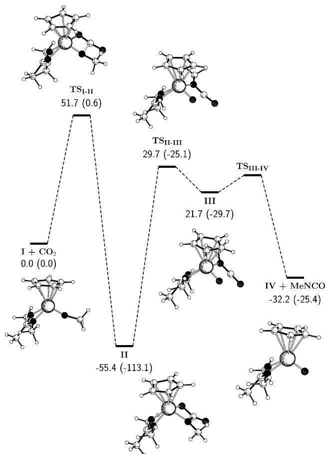
Figure 6. DFT computed pathway for the reaction of [\text{Ti}(\eta\text{-C}_5\text{H}_5)(\text{NMe})\{\text{MeC}(\text{NMe})_2\}] ( I ) with CO 2 showing Gibbs free energies at 298 K (kJ mol -1 ). Electronic energies are given in parentheses. Representations of the DFT structures are shown (left to right) for I , TS I-II , II , TS II-III , III , and IV . See the text for further details.
