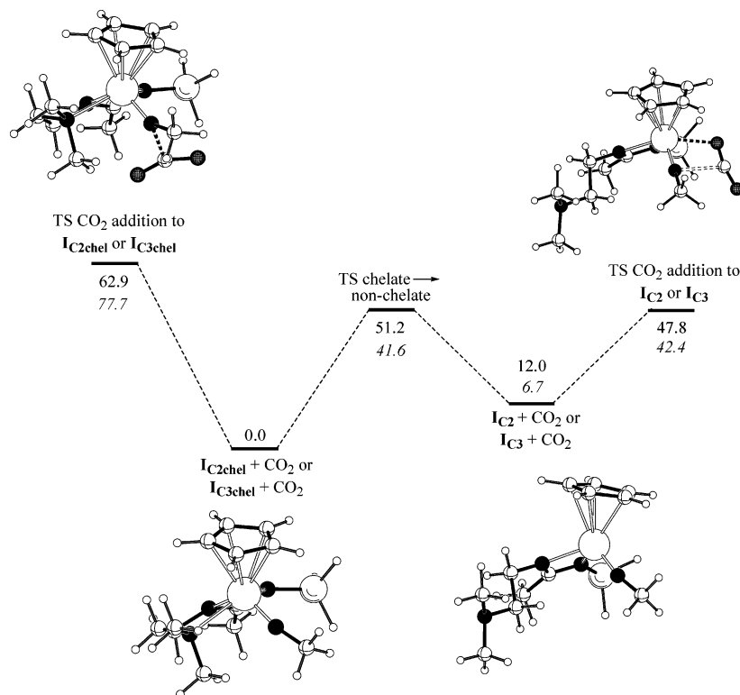
Figure 10. Schematic representation of free energies for CO 2 addition for both the chelated and nonchelated imido–amidinate systems at 200 K, relative to the respective chelated isomers. The upper value in each pair is for the two-carbon arm system and the lower value (in italics) is for the three-carbon arm systems (TS = transition state). All energies are from DFT calculations except for “TS chelate → nonchelate” which are derived from the \Delta H^\ddagger and \Delta S^\ddagger data for 3 and 4 (Table 1). DFT minimized geometries for the two-carbon arm system are illustrated.
