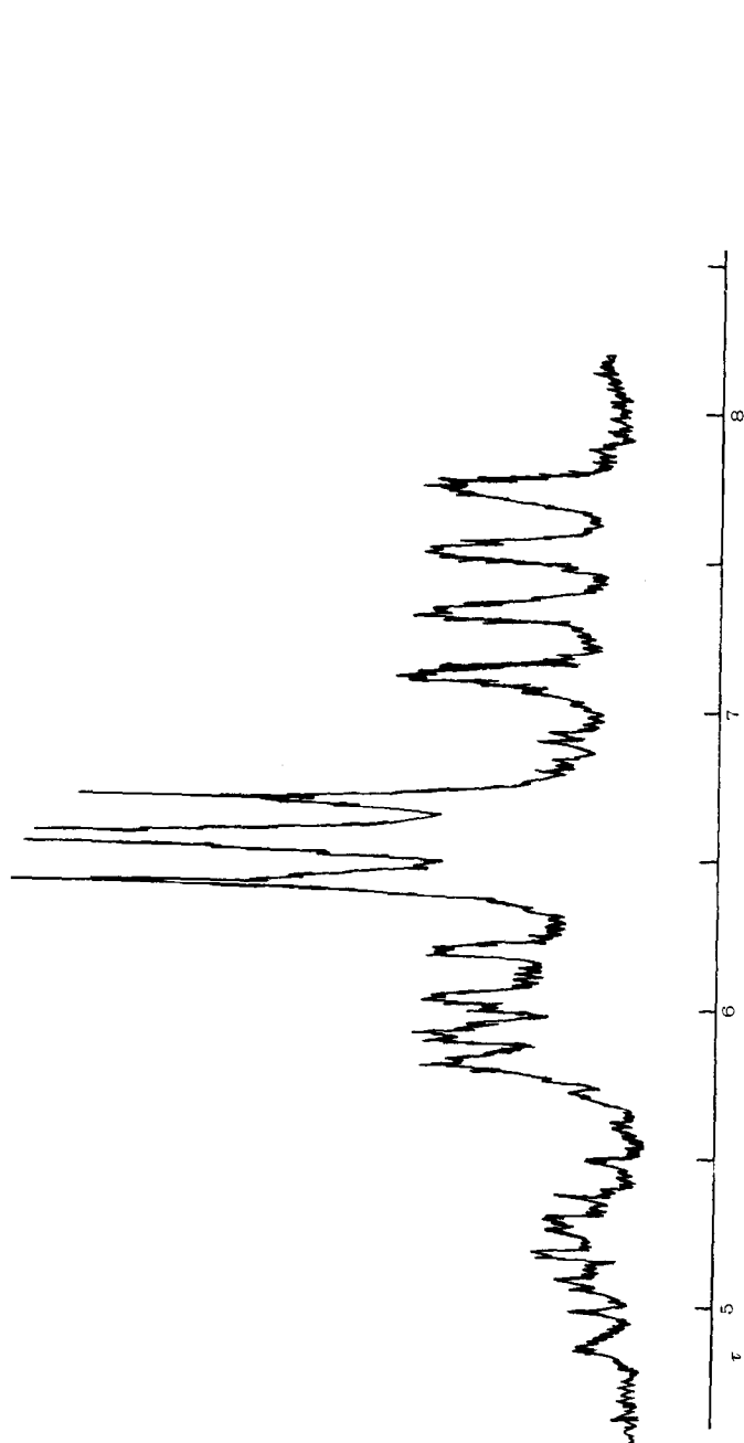
Figure 1. PMR spectrum at 60 MHz in \text{CDCl}_3 solution of [\text{Pt}(\eta^3\text{-allyl})(\text{CH}_3\text{NC})\text{Cl}] .
