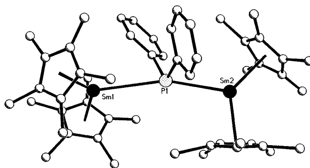
Figure 5. Structure of (\text{C}_5\text{Me}_5)_2\text{Sm}(\mu\text{-PPh}_2)\text{Sm}(\text{C}_5\text{Me}_5)_2 , 7 .
