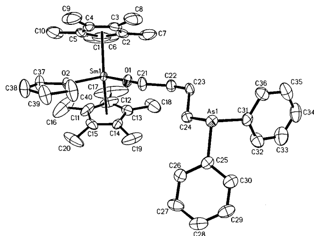
Figure 4. Thermal ellipsoid plot of (\text{C}_5\text{Me}_5)_2\text{Sm}[\text{O}(\text{CH}_2)_4\text{AsPh}_2](\text{THF}) , 6 , with ellipsoids drawn at the 50% probability level.
