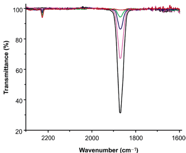
Figure 1. IR spectroscopic monitoring of the reaction between an equimolar ratio of 1 and hydrazine in methanol at 20 °C. Complex 1 without (black) and with hydrazine after 6 min (magenta), 12 min (blue), 18 min (green), and 25 min (red).
