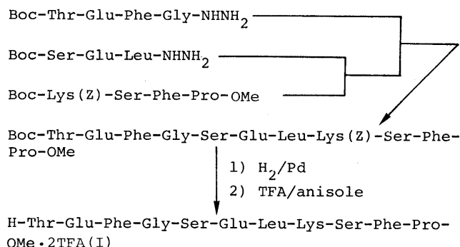
Fig. 2. Synthetic Scheme for H-(1-11)-OMe (I)
