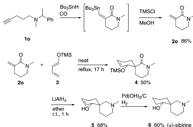
Scheme 4. Carbonylative S_{\text{H}}\text{I} -Type Reaction of a Tertiary Alkynylamine 1o and Its Application to the Synthesis of ( \pm )-Sibirine
