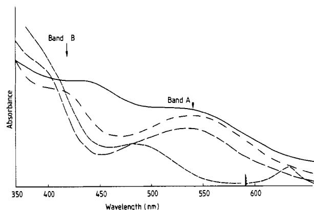
Figure 5. Visible spectra, in \text{CH}_2\text{Cl}_2 , of (i) (---) 1 , (ii) (—) 1 + , (iii) (—) \text{ClCCO}_3(\text{CO})_9 , and (iv) (---) [\text{FcCCO}_3(\text{CO})_9\text{P}(\text{C}_6\text{H}_{11})_3]^+ (change of absorbance scale at 580 nm).
