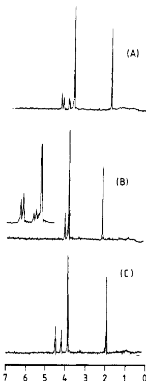
Figure 2. 1 H NMR of regioisomers of (Me)Fc(CO)CCo 3 (CO) 9 (in CDCl 3 ): (A) 1,2; (B) 1,3; (C) 1,1'.
