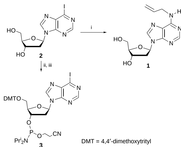
Scheme 1 Reagents and conditions: i, allylamine (neat), room temp.; ii, 4,4'-dimethoxytrityl chloride, Pr i 2 EtN, CH 2 Cl 2 ; iii, N,N-diisopropyl-O-cyanoethylphosphoramidic chloride, Pr i 2 EtN, CH 2 Cl 2
