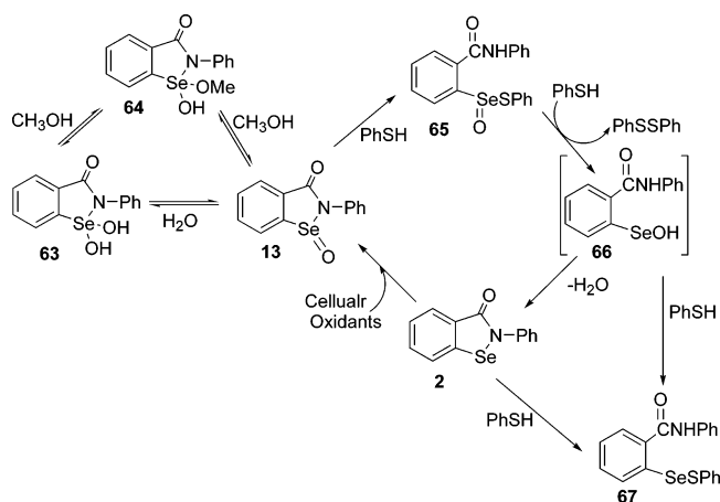
Scheme 7. Proposed Mechanism for the Reduction of Selenoxide 48 to Selenide 20
