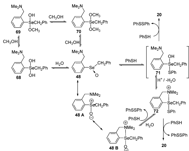
Scheme 7. Proposed Mechanism for the Reduction of Selenoxide 48 to Selenide 20
