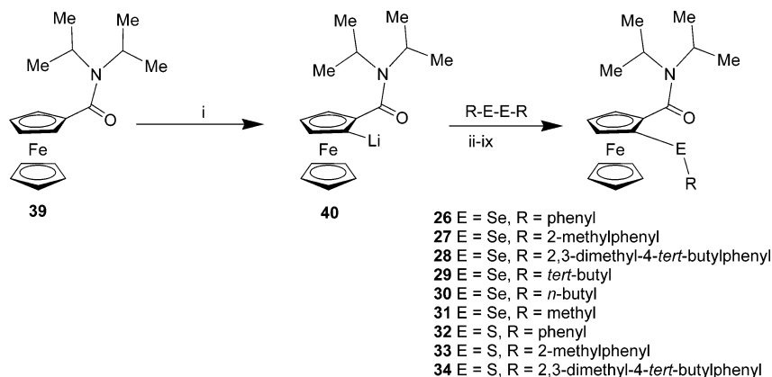
Scheme 3. Synthesis of Selenides/Sulfides ( 26–34 ) a
