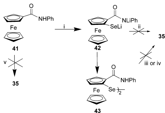
Scheme 4. Attempted Synthesis of Ferrocene-Ebselen ( 35 ) a
