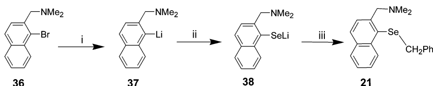
Scheme 2. Synthesis of Selenide 21 a
