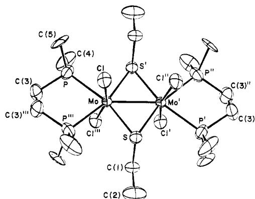
Figure 2. An ORTEP view of the \text{Mo}_2(\mu\text{-SEt})_2\text{Cl}_4(\text{dmpe})_2 molecule in compound 2. Thermal ellipsoids enclose 50% of the electron density. Singly primed, doubly primed, and triply primed atoms are related to unprimed atoms by an inversion center, mirror plane, and a twofold axis, respectively.
