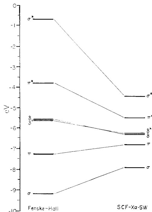
Figure 8. A comparison of the results of the Fenske-Hall calculation and an SCF-Xα-SW calculation on Mo 2 Cl 4 (μ-SH) 2 (SH 2 ) 4 , both done at the Mo-Mo distance of 2.68 Å.
