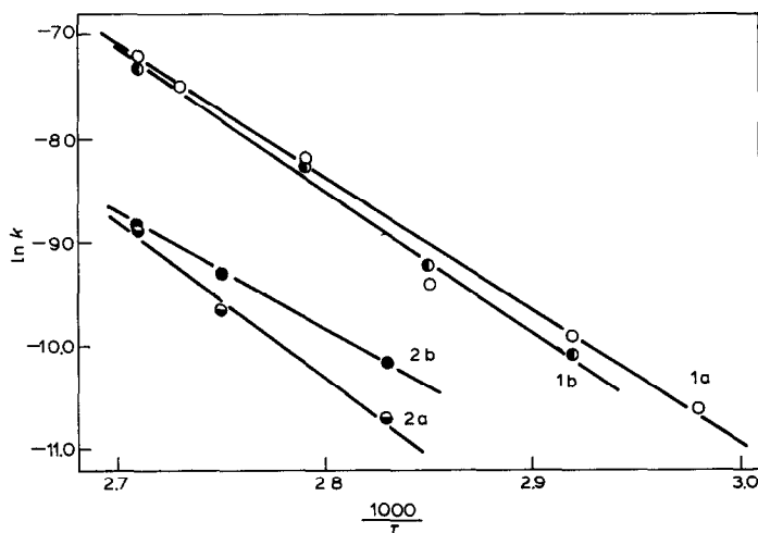
Fig. 22. Plots of \ln k for the reactions of formation (a) and para-meta isomerisation (b) of the \sigma -tolyl complex of Pt^{IV} in CF 3 COOH/H 2 O (1) (see Fig. 2) and CH 3 COOH/H 2 O (2) (see Fig. 3) vs. 1/T .
