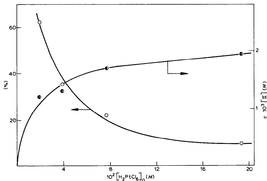
Fig. 25. Plots of the yield and concentration c (M) of complex II in the photoinduced reaction of \text{H}_2\text{PtCl}_6 with anisole ( 0.64 M ) in \text{CH}_3\text{COOH} (50 min reaction time) vs. the initial concentration of \text{PtCl}_6^{2-} .
