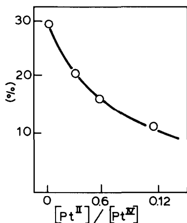
Fig. 31. Plot of the yield of complex II in the photoinduced reaction of \text{H}_2\text{PtCl}_6 (0.077 M ) with anisole (0.64 M ) in \text{CH}_3\text{COOH}/\text{H}_2\text{O} (21/1 v/v) (50 min reaction time) vs. the relative concentration of \text{Na}_2\text{PtCl}_4 added (with respect to \text{Pt}^{\text{IV}} ).
