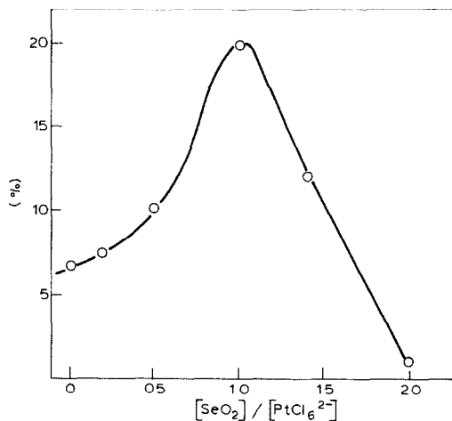
Fig. 16. Plot of the yield of complex II in the thermal reaction of \text{H}_2\text{PtCl}_6 ( 0.17\text{ M} ) with benzene ( 1.9\text{ M} ) in \text{CH}_3\text{COOH} at 80^\circ\text{C} (2 h reaction time) vs. the concentration of \text{SeO}_2 added.
