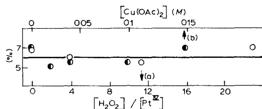
Fig. 19. Plots of the yield of complex II in the thermal reaction of \text{H}_2\text{PtCl}_6 (0.17 M) with benzene (1.9 M) in \text{CH}_3\text{COOH} at 80^\circ\text{C} (2 h reaction time) vs. the concentration of \text{H}_2\text{O}_2 (a) or \text{Cu}(\text{OAc})_2 (b) added.
