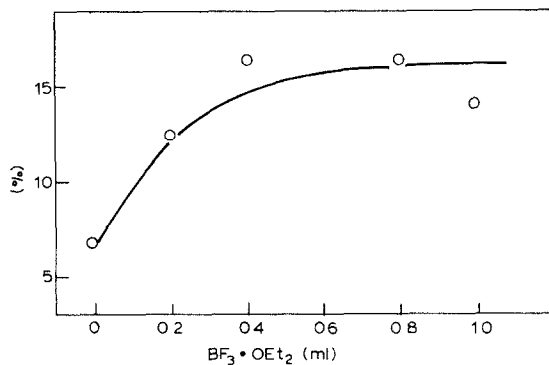
Fig. 14. Plot of the yield of complex II in the thermal reaction of \text{H}_2\text{PtCl}_6 ( 0.17\text{ M} ) with benzene ( 1.9\text{ M} ) in \text{CH}_3\text{COOH} ( 80^\circ\text{C} , 2 h reaction time) vs. \text{BF}_3 \cdot \text{OEt}_2 added. Total volume of reaction mixture 5 ml.
