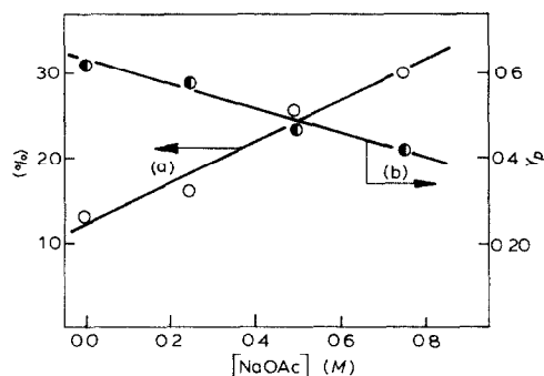
Fig. 15. Plots of the yield of complex II (a) and the relative content of p -isomer Y_p (b) in the thermal reaction of \text{H}_2\text{PtCl}_6 ( 8.05 \times 10^{-2}\text{ M} ) with toluene ( 0.73\text{ M} ) at 90^\circ\text{C} (50 min reaction time) vs. [\text{NaOAc}] added.
