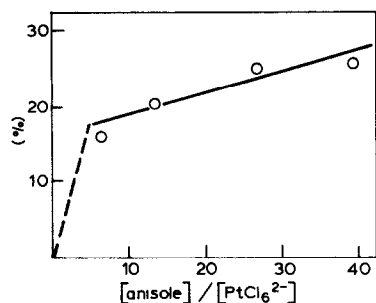
Fig. 26. Plot of the yield of complex II in the photoinduced reaction of \text{H}_2\text{PtCl}_6 ( 0.077 M ) with anisole in \text{CH}_3\text{COOH} (50 min reaction time) vs. the relative concentration of anisole (with respect to \text{Pt}^{\text{IV}} ).
