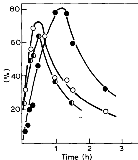
Fig. 13. Plots of the yield of complex II in the thermal reaction of \text{H}_2\text{PtCl}_6 (0.074 M ) with benzene (2.2 M ) in \text{CF}_3\text{COOH}/\text{H}_2\text{O} (6/1 v/v) vs. time. (●) Without additives; (○) \text{Na}_2\text{PtCl}_4 (0.025 M ) added; (◐) \text{Hg}(\text{OAc})_2 (0.014 M ) added.
