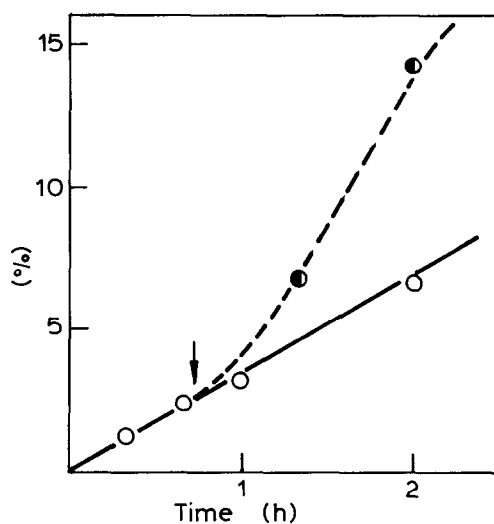
Fig. 17. Plot of the yield of complex II in the thermal reaction of \text{H}_2\text{PtCl}_6 (0.17 M) with benzene (1.9 M) in \text{CH}_3\text{COOH} at 79.5^\circ\text{C} . (○) Without additives and (●) with p -quinone ( 8.3 \times 10^{-3} M) added at 45 min reaction time (denoted by an arrow) vs. time.
