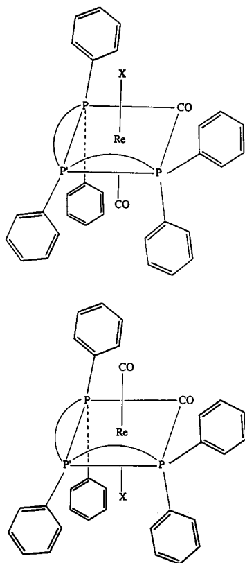
Figure 7. Diagrammatic representations of the two isomers of cis,mer - Re(CO)_2(P_2P')Cl .
