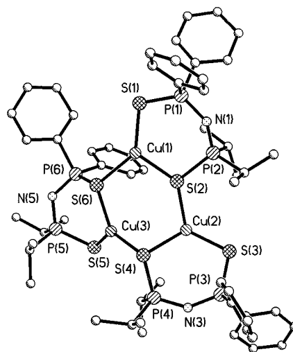
Figure 3. X-ray structure of [Cu I ( t Pr 2 P(S)NP(S)Ph 2 ) 3 ] ( 3 ).
