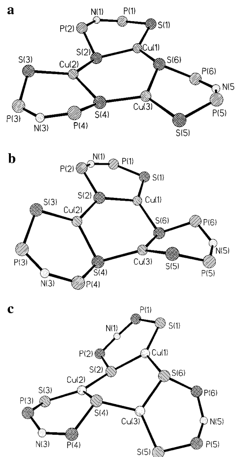
Figure 2. X-ray structure of the core geometries in (a) [Cu I N( i Pr 2 P(S)NP(S)(OPh) 2 ) 3 ] (1), (b) [Cu I ( i Pr 2 P(S)NP(S)(OPh) 2 ) 3 ] (3), and (c) [Cu I ( i Pr 2 P(S)NP(S)(OPh) 2 ) 3 ] (4).
