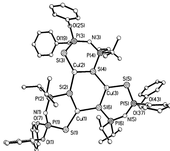
Figure 4. X-ray structure of [Cu I ( t Pr 2 P(S)NP(S)(OPh) 2 ) 3 ] ( 4 ).
