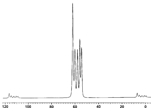
Figure 1. Solid state ^{31}\text{P} NMR spectrum of 1.
