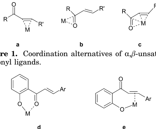
Figure 2. Coordination of chalcone ligands.
