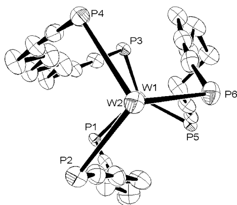
Figure 4. Projection of 5 down the \text{W2-W1} vector to show the paddle-wheel arrangement of the ligands.
