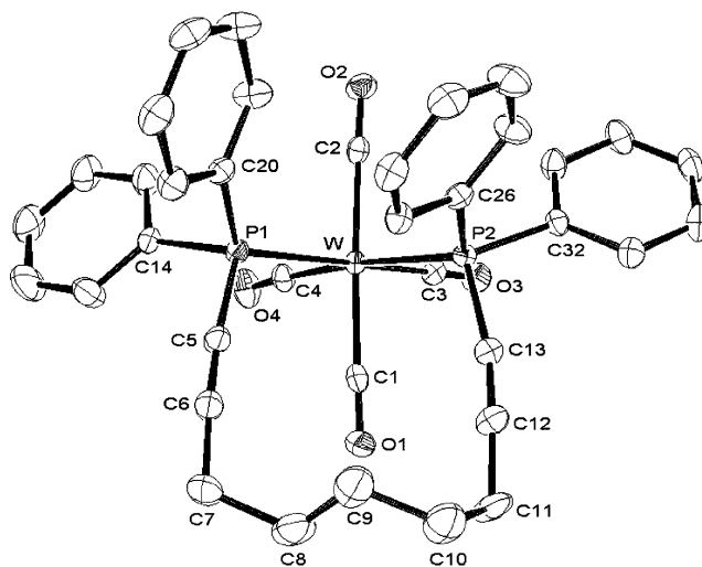
Figure 2. Molecular structure of 2 . Selected bond distances (Å): \text{W--P}1 = 2.5255(7) , \text{W--P}2 = 2.5150(6) , \text{W--C}1 = 2.034(3) , \text{W--C}2 = 2.026(3) , \text{W--C}3 = 1.982(3) , \text{W--C}4 = 2.000(3) , \text{C}5\text{--C}6 = 1.193(4) , \text{C}12\text{--C}13 = 1.190(4) . Selected bond angles (deg): \text{P}1\text{--W--P}2 = 98.56(2) , \text{P}1\text{--W--C}3 = 174.27(7) , \text{P}2\text{--W--C}4 = 172.75(8) , \text{C}1\text{--W--C}2 = 177.7(1) , \text{C}5\text{--P}1\text{--W} = 112.70(9) , \text{C}6\text{--C}5\text{--P}1 = 174.3(3) , \text{C}5\text{--C}6\text{--C}7 = 176.0(3) , \text{C}13\text{--P}2\text{--W} = 111.82(9) , \text{C}12\text{--C}13\text{--P}2 = 169.4(3) , \text{C}13\text{--C}12\text{--C}11 = 177.3(3) .
