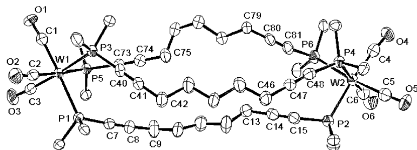
Figure 3. Molecular structure of 5 . The \text{C}_6\text{H}_5 groups have been artificially omitted, except the ipso carbon atoms, for clarity. Selected bond distances (Å): \text{W1-P1} = 2.528(2) , \text{W1-P3} = 2.532(2) , \text{W1-P5} = 2.525(2) , \text{W1-C1} = 1.978(7) , \text{W1-C2} = 1.966(8) , \text{W1-C3} = 1.969(7) , \text{W2-P2} = 2.507(2) , \text{W2-P4} = 2.535(2) , \text{W2-P6} = 2.529(2) , \text{W2-C4} = 1.950(8) , \text{W2-C5} = 1.989(8) , \text{W2-C6} = 1.946(8) . Selected bond angles (deg): \text{P1-W1-P3} = 90.62(5) , \text{P1-W1-P5} = 90.63(6) , \text{P3-W1-P5} = 94.98(6) , \text{P2-W2-P4} = 171.8(2) , \text{P6-W2-C5} = 172.4(2) , \text{P4-W2-C6} = 177.6(2) , \text{P2-W2-P6} = 92.86(6) , \text{P2-W2-P4} = 94.01(6) , \text{P4-W2-P6} = 89.11(6) , \text{C8-C7-P1} = 177.1(6) , \text{C7-C8-C9} = 176.1(8) , \text{C14-C15-P2} = 167.1(7) , \text{C13-C14-C15} = 177.8(8) , \text{C41-C40-P3} = 178.1(7) , \text{C40-C41-C42} = 178.4(8) , \text{C47-C48-P4} = 173.2(6) , \text{C46-C47-C48} = 177.7(8) , \text{C74-C73-P5} = 168.3(7) , \text{C73-C74-C75} = 174.5(9) , \text{C80-C81-P6} = 173.1(6) , \text{C79-C80-C81} = 176.4(7) .
