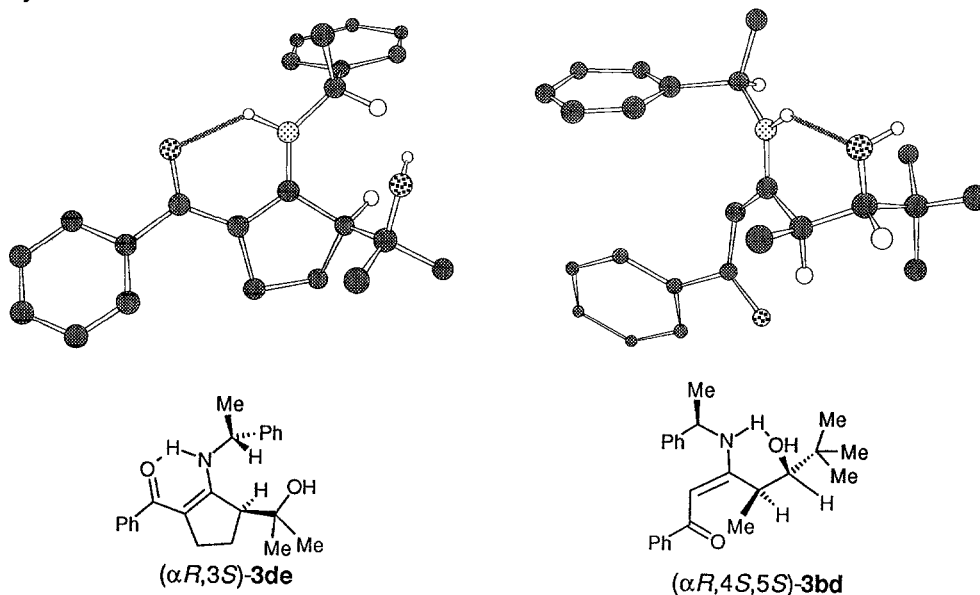
Figure 2. Ball and stick depiction of X-ray of the single crystal structures of cyclic ( \alpha R,3S )- 3de and acyclic ( \alpha R,4S,5S )- 3bd \delta -hydroxy enaminones. Most of the hydrogen atoms have been omitted for clarity.
