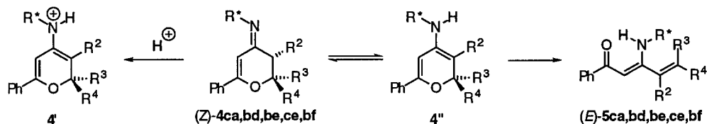
Scheme 5. Electrocyclic rearrangement of 4-imino-2,3-dihydropyranones to \gamma -alkyldenaminones 5.
