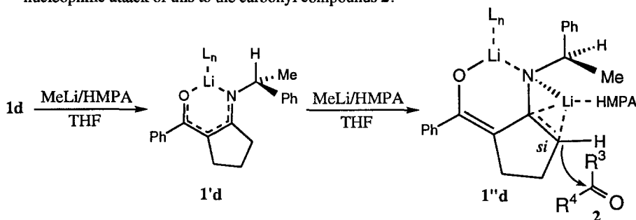
Scheme 1. Formation process of the chiral enaminone lithium dianion 1''d and nucleophilic attack of this to the carbonyl compounds 2 .
