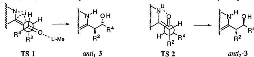
Scheme 2 - The more probable transition state ( Ts 1 ) and the chelation control transition state ( Ts 2 ) for the nucleophilic attack of lithium dianion 1''d to the carbonyl compounds 2 .
