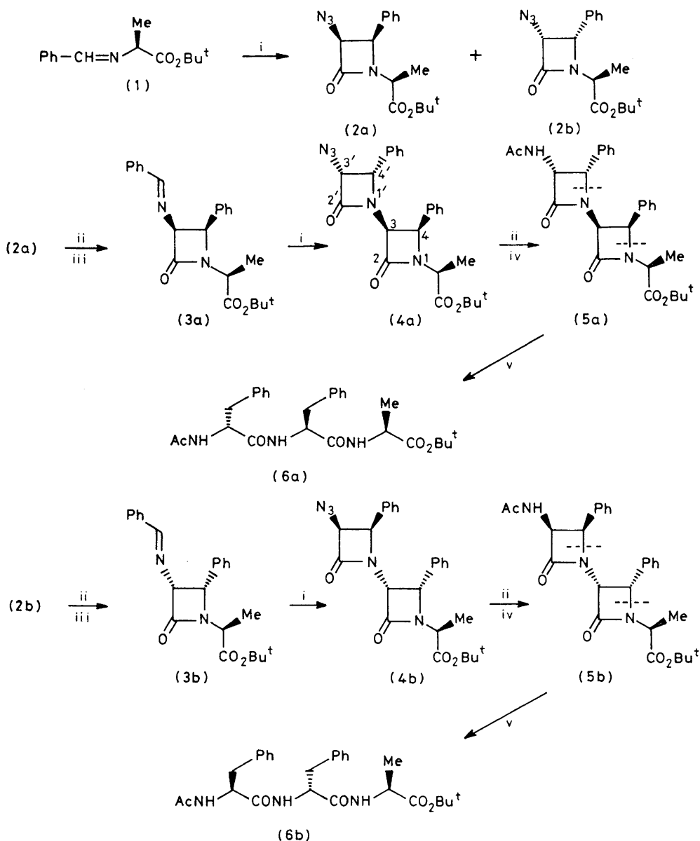
SCHEME. Asymmetric synthesis of bis- \beta -lactams; i, \text{N}_3\text{CH}_2\text{COCl} , \text{Et}_3\text{N} , \text{CH}_2\text{Cl}_2 , -78^\circ\text{C} to room temperature; ii, \text{H}_2 (1 atm), 5% Pd-C, MeOH, room temperature; iii, \text{PhCHO} , \text{MgSO}_4 , \text{PhH} ; iv, \text{Ac}_2\text{O} , N -methylmorpholine, \text{CHCl}_3 ; v, \text{H}_2 (1 atm), 10% Pd-C, EtOH, 50^\circ\text{C} .
