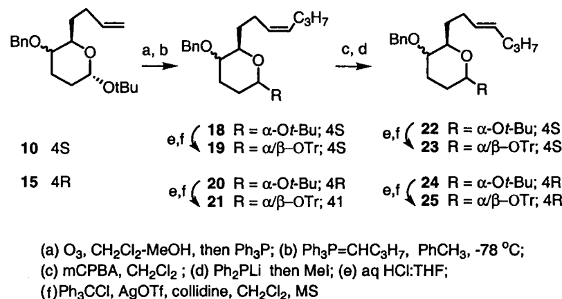
Scheme 4. Synthesis of Z- and E-alkenes.
