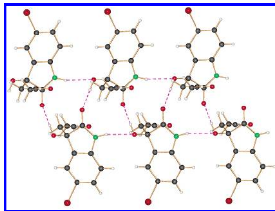
FIGURE 4. Crystal packing of 1e showing the zigzag chain generated by the intermolecular hydrogen bonds running along the b -axis.
