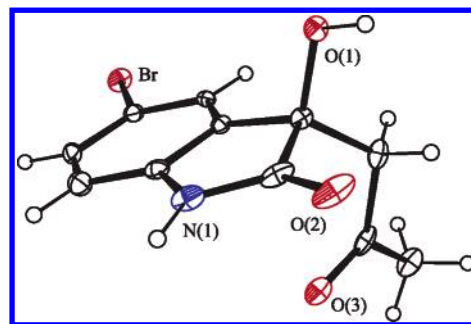
FIGURE 3. ORTEP drawing of the ( R )-enantiomer of 1e (30% thermal ellipsoids).
