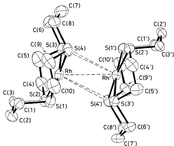
Figure 1. ORTEP drawing (50% probability ellipsoids) showing the dimeric structure of the cation \{\text{Rh}[14]\text{aneS}_4\}^+ (1). Principal distances and angles (e.s.d.s. in parentheses): Rh–S(1) 2.285(4), Rh–S(2) 2.282(5), Rh–S(3) 2.261(3), Rh–S(4) 2.264(6) Å; S(1)–Rh–S(2) 87.3(1), S(2)–Rh–S(3) 88.1(1), S(3)–Rh–S(4) 95.8(1), S(4)–Rh–S(1) 87.9(1)°.
