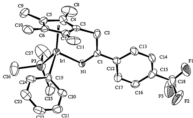
Figure 2. ORTEP diagram of \text{Ph(PMe}_3\text{)Ir[C}_5\text{Me}_4\text{CH}_2\text{C(C}_6\text{H}_4\text{CF}_3\text{)N]} ( 12 ). Hydrogen atoms have been omitted for clarity. Thermal ellipsoids are shown at 50% probability.
