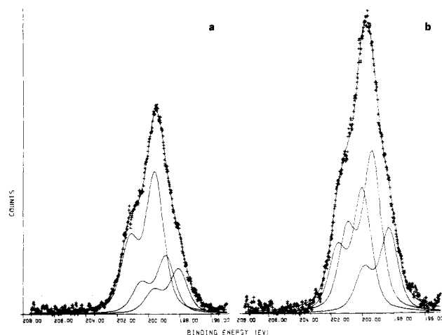
Figure 1. Cl 2p_{3/2} XPS of [\text{Mo}_4\text{Cl}_8(\text{PEt}_3)_2]_x : (a) scans 1–20; (b) scans 51–70. The sum of the resolved components is given by the solid line through the data points.
