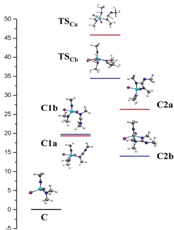
Figure 5. Comparison between the relative free energy ( kcal\cdot mol^{-1} ) profile for the carbodiimide addition to the V–imido bond (red) and the carbodiimide insertion into the V–amido bond (blue) in toluene.
