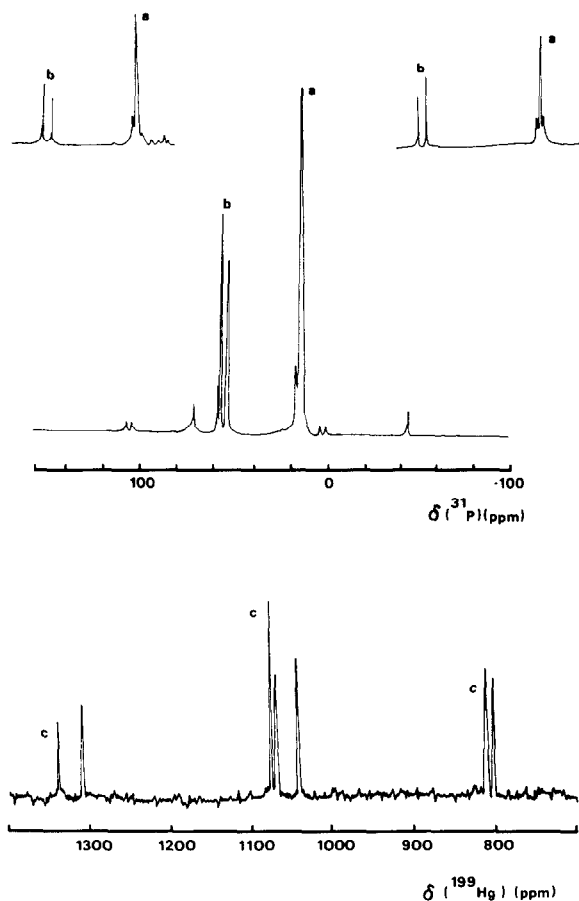
Fig. 1. Phosphorus-31 and mercury-199 spectra at -50^{\circ}\text{C} of a 1:1 solution of \text{HgCl}_2(\text{HPcycl}_2)_2 and \text{C}_6\text{H}_5\text{NCS} . Regions a and b are associated with the phosphorus resonances of coordinated \text{HPcycl}_2 and \text{LH} respectively. c is the triplet due to \text{HgCl}_2(\text{HPcycl}_2)_2 and the doublet of doublets is assigned as due to the mixed ligand species \text{HgCl}_2(\text{HPcycl}_2)(\text{LH}) .
