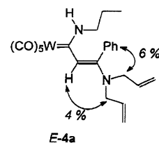
Fig. 2. Results of the nuclear overhauser experiment with E-ua.
