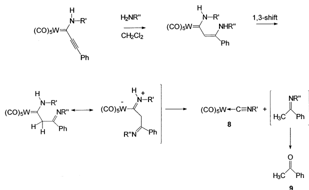
Scheme 2. Reaction of allylamine with complex 1b .
