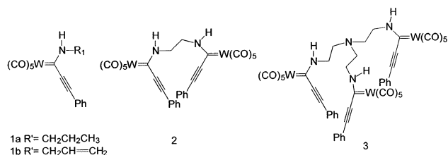
Fig. 1. Amino carbene complexes 1–3.
