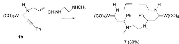
Scheme 1. Reaction of N,N' -dimethylethylenediamine with complex 1b .
