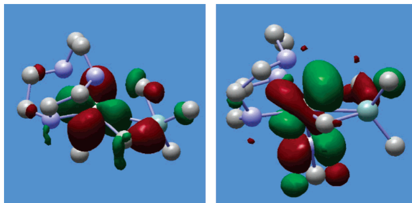
Figure 11. LUMO (left) and LUMO+1 (right) for [Ti(NMe)(H 3 [9]aneN 3 )(CH 2 SiMe 3 ) + ( 7q ). H atoms omitted for clarity.
