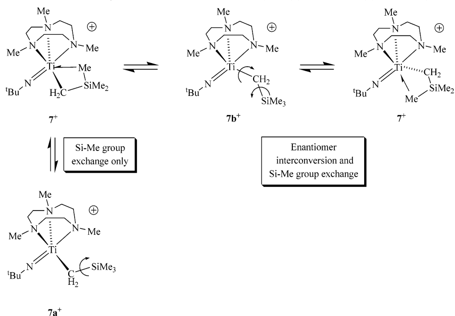
Scheme 3. Reaction of \text{Ti}(\text{N}^t\text{Bu})(\text{Me}_3[9]\text{aneN}_3)\text{Cl}(\text{Me}) with [\text{Ph}_3\text{C}][\text{BAR}^F_4] and Subsequent Trapping of the in Situ-Generated [\text{Ti}(\text{N}^t\text{Bu})(\text{Me}_3[9]\text{aneN}_3)\text{Cl}]^+ Cation a
