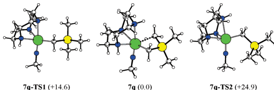
Figure 10. DFT(B3PW91)-optimized geometries and relative energies (kJ mol -1 ) for 7q-TS1 (left), 7q (center), and 7q-TS2 (right).
