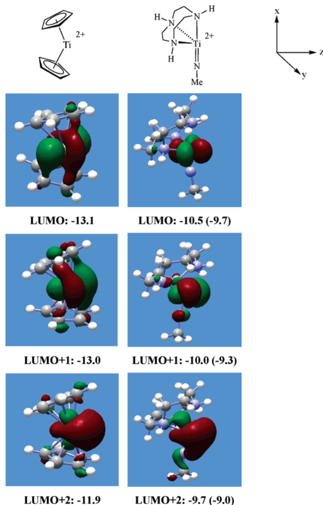
Figure 7. Three lowest unoccupied MOs for [Cp_2Ti]^{2+} (II, left) and [Ti(NMe)(H_3[9]aneN_3)]^{2+} (I, right), their corresponding energies (eV), and the chosen coordinate system. Values for [Ti(N^tBu)(Me_3[9]aneN_3)]^{2+} (V) are given in parentheses.
