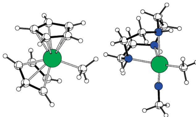
Figure 9. DFT(B3PW91)-optimized geometry for [\text{Cp}_2\text{TiMe}]^+ (left) and [\text{Ti}(\text{NMe})(\text{H}_3[9]\text{aneN}_3)\text{Me}]^+ ( 6q , right).
