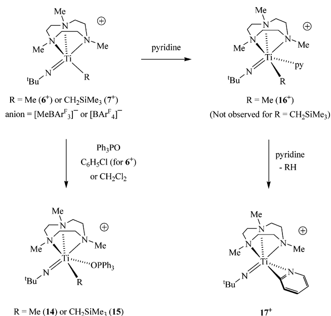
Scheme 6. Reactions of [\text{Ti}(\text{N}^t\text{Bu})(\text{Me}_3[9]\text{aneN}_3)\text{R}]^+ ( \text{R} = \text{Me} or \text{CH}_2\text{SiMe}_3 ) with \text{Ph}_3\text{PO} and Pyridine a
