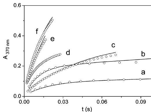
Figure 6. Experimental (O) and fitted (—) kinetic traces at pH = 1.50: [HOBr] 0 = 1.0 \times 10^{-4} M, [Cl(III)] 0 = 2.0 \times 10^{-3} M (a); [HOBr] 0 = 2.0 \times 10^{-4} M, [Cl(III)] 0 = 3.0 \times 10^{-3} M (b); [HOBr] 0 = 1.0 \times 10^{-3} M, [Cl(III)] 0 = 4.0 \times 10^{-4} M (c); [HOBr] 0 = 4.0 \times 10^{-3} M, [Cl(III)] 0 = 2.0 \times 10^{-4} M (d); [HOBr] 0 = 6.0 \times 10^{-4} M, [Cl(III)] 0 = 2.0 \times 10^{-3} M (e); [HOBr] 0 = 2.0 \times 10^{-3} M, [Cl(III)] 0 = 8.0 \times 10^{-4} M (f); T = 25 °C, I = 1.0 M. For sake of simplicity, only a portion of the experimental data points is shown in each experimental trace.
