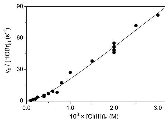
Figure 4. The normalized initial rate as a function of [\text{Cl(III)}] at constant pH. Solid line (—): fitted curve on the basis of eq 8. [\text{HOBr}]_0 = (0.1\text{--}2.0) \times 10^{-3} \text{ M} , pH = 1.50. T = 25^\circ \text{C} , I = 1.0 \text{ M} .
