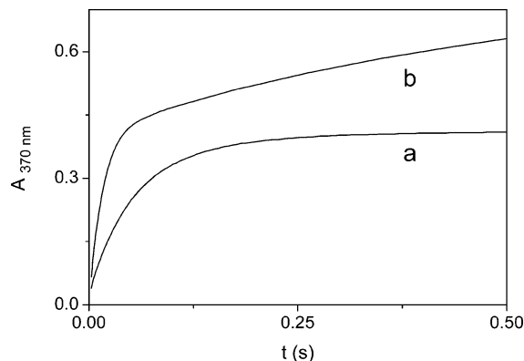
Figure 2. Typical kinetic traces at HOBr excess: [\text{HOBr}]_0 = 1.0 \times 10^{-3} \text{ M} , [\text{Cl(III)}]_0 = 4.0 \times 10^{-4} \text{ M} , \text{pH} = 1.50 (a). At Cl(III) excess: [\text{HOBr}]_0 = 4.0 \times 10^{-4} \text{ M} , [\text{Cl(III)}]_0 = 2.0 \times 10^{-3} \text{ M} , \text{pH} = 1.50 (b). T = 25^\circ \text{C} , I = 1.0 \text{ M} .
