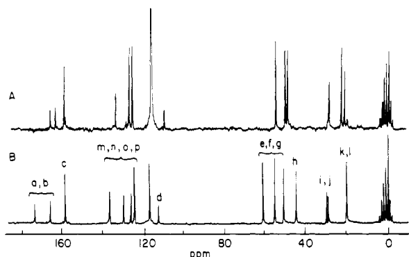
Figure 2. Carbon-13 NMR spectra for the complexes: A, [Ni(( p -xylyl)(NHEthi) 2 Me 2 [16]tetraeneN 4 )](PF 6 ) 2 ; B, [Ni(( m -xylyl)(MeNEthi) 2 Me 2 [16]tetraeneN 4 )](PF 6 ) 2 . For meaning of labels, see structure VIII.
