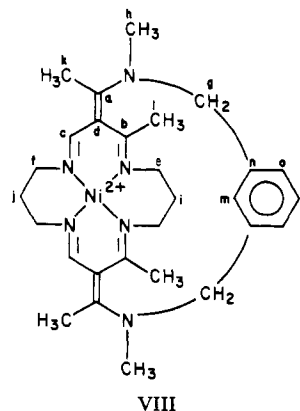
Figure 2b for [Ni(( m -xyl)(MeNEthi) 2 [16]tetraeneN 4 )](PF 6 ) 2 .
