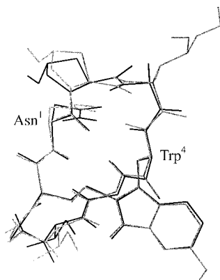
Figure 7. Superposition of the structures of S-deoxo-Ala³-amaninamide (black line) and β-amanitin (gray line).
