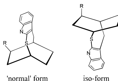
Figure 3. Schematic drawing of the two possible isomers for amatoxins.
