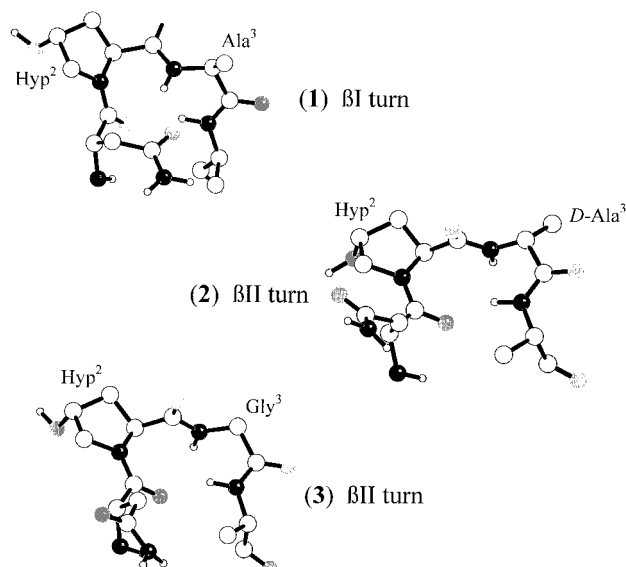
Figure 8. Structures of the turns with Hyp² in the i +1 position in all three analogues.
