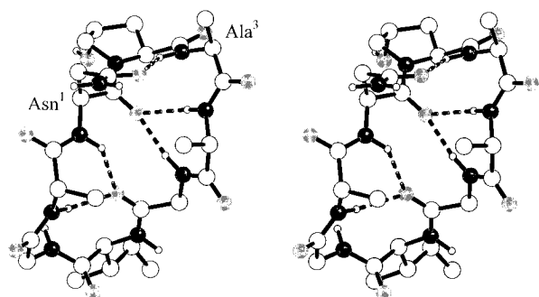
Figure 6. Stereoscopic picture of the backbone conformation of S-deoxo-Ala³-amaninamide ( 3 ); hydrogen bonds are painted as dashed lines.
