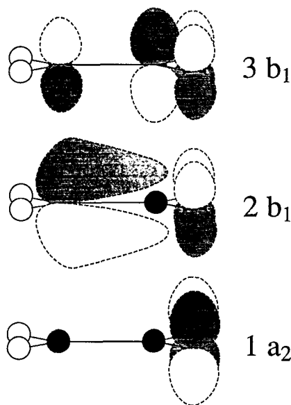
FIG. 7. A form of the 1a_2 , 2b_1 , and 3b_1 molecular orbitals determined from ab initio calculations performed on \text{CH}_2\text{NO}_5^- .
