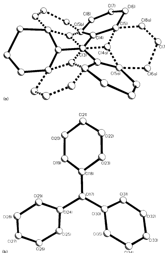
Fig. 3. The structure of the anion [\text{Ph}_3\text{C}]^- in 1 (a) (one of the disordered [\text{Ph}_3\text{C}]^- fragments is shown in dashed solid line) and in 2 (b).
