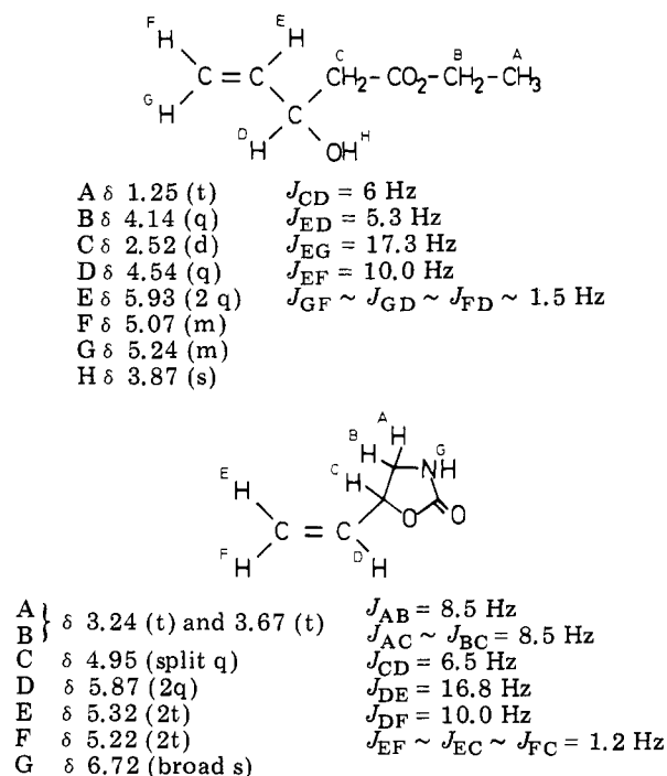
Figure 5. NMR spectral data for ethyl 3-hydroxypentenate (60 MHz, CDCl 3 ) and 5-vinylloxazolidinone (100 MHz, CDCl 3 ).
