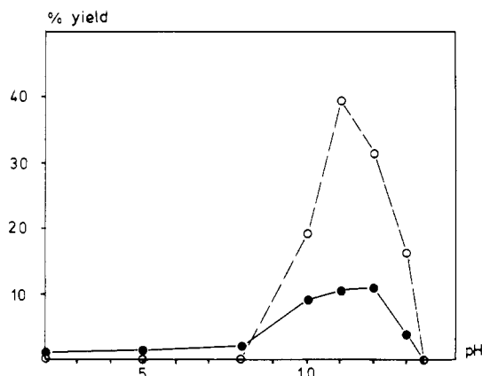
Figure 4. Yield of 1-cyano-2-hydroxy-3-butene (●) and 5-vinyloxazolidinone (○) in the hydrolysis of progoitrin at 100 °C at various pHs in the presence of sodium tetraborate buffer.
