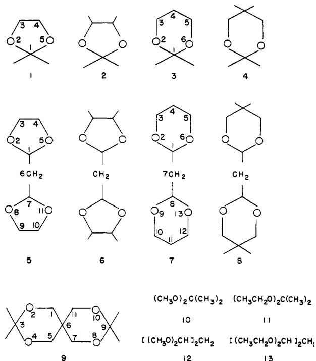
Figure 1. Acetal and ketal structures
