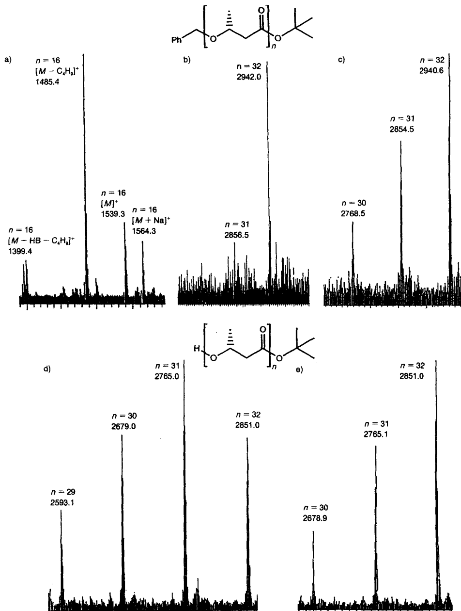
Fig. 1. FAB Mass spectra of samples of the fully protected 16mer 4a , the 32mer 5a , and of the debenzilation product 5c . All spectra were obtained such that the measured ions had the (M + \text{Na}) masses, except the 16mer 4a in part a . The signals at 1400 Da are due to fragmentation of the 16mer, because essentially no signals for the M^+ of the protected 15mer are visible. a ) 16mer 4a . b ) and c ) 32mer 5a obtained from two different runs, with the sample for b prepared with debenzilation of the 16mer 4a in \text{CF}_3\text{CH}_2\text{OH} , for c in \text{HCONMe}_2 (DMF). d ) Product of debenzilation of 5a in DMF ( 70^\circ to 20^\circ ), e ) in \text{CF}_3\text{CH}_2\text{OH} . As can be seen by comparing b with c , and d with e , the loss of HB units occurs especially in DMF as a solvent and at elevated temperatures.
