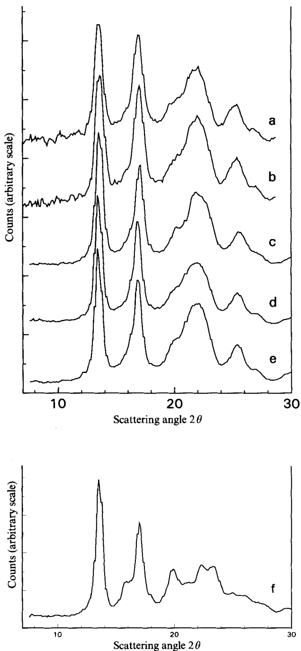
Fig. 7. WAXS Profiles of a) P (3- HB ) ( 1 ), b) bacterial P (3- HB ) after degradation with Li base, c) the 16mer after removal of the protecting end groups ( 4d ), d) the fully protected 16mer ( 4a ), e) the fully protected 32mer of 3- HB ( 5a ). Apart from minor differences caused by changes in crystallinity and crystal perfection, all the patterns are the same. f) Distinctly different WAXS profile of 8mer 3d .
