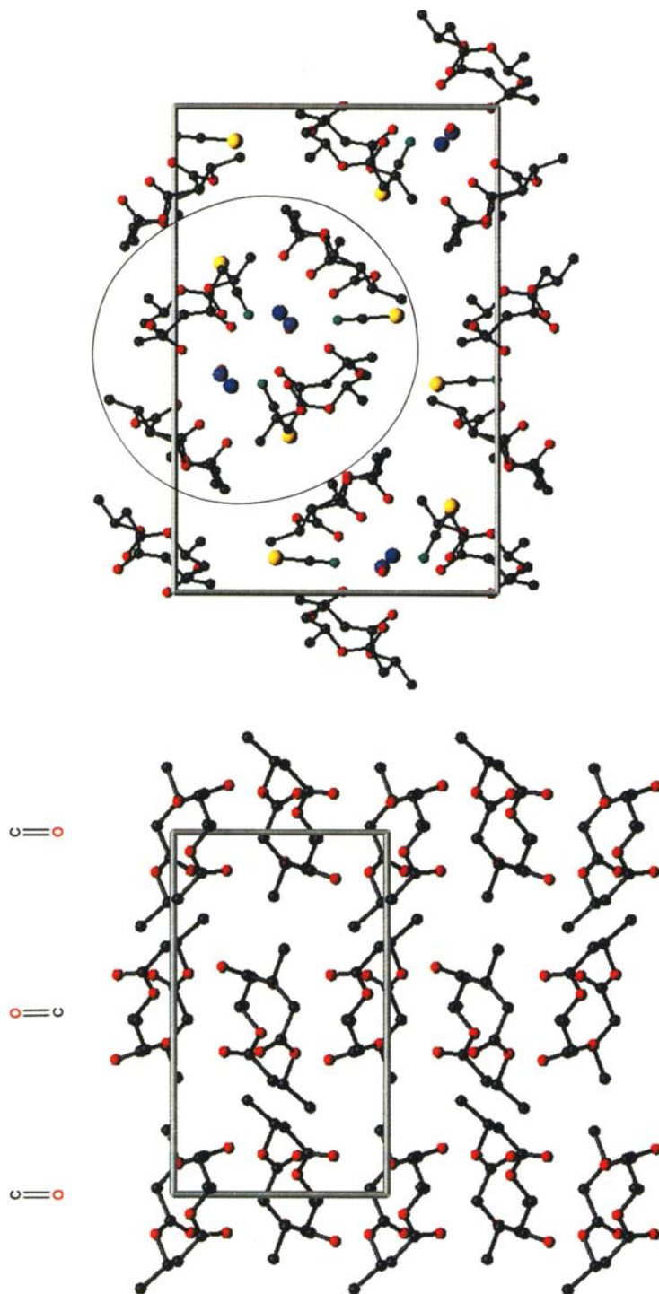
Fig. 10. Sections from the crystal structures of the cyclic trimer of 3-HB, a triolide (left), and of the triolide complex with KSCN (2 KSCN · 2 triolide · H 2 O). The triolide molecules form sheets with the C=O groups aligned parallel in opposite directions on neighboring layers (left). In the complex, the triolide molecules rally round the K + ions, and formally a channel is formed with the K + ions inside, and the SCN - N-atoms and triolide carbonyl O-atoms assembled along the inner wall. The outside of this channel may be considered lipophilic. For a discussion and comparison with similar complexes of NaSCN and Ba(SCN) 2 , see [35].
